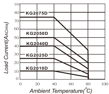
Load Current VS. Ambient Temp.
